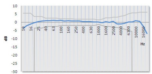
Free field response with Z weighting
